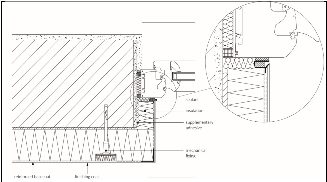
Figure 9 Insulated reveal detail
